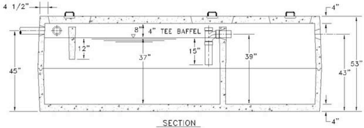
COMBINATION 1000 GALLON & 500 GALLON PUMP TANK
