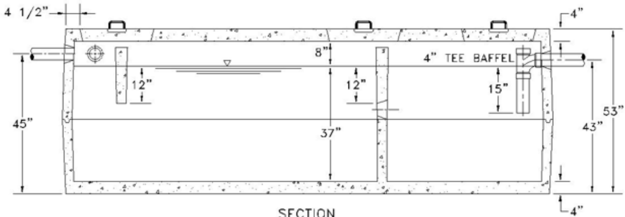
1500 GALLON 2 COMPARTMENT SEPTIC TANK
